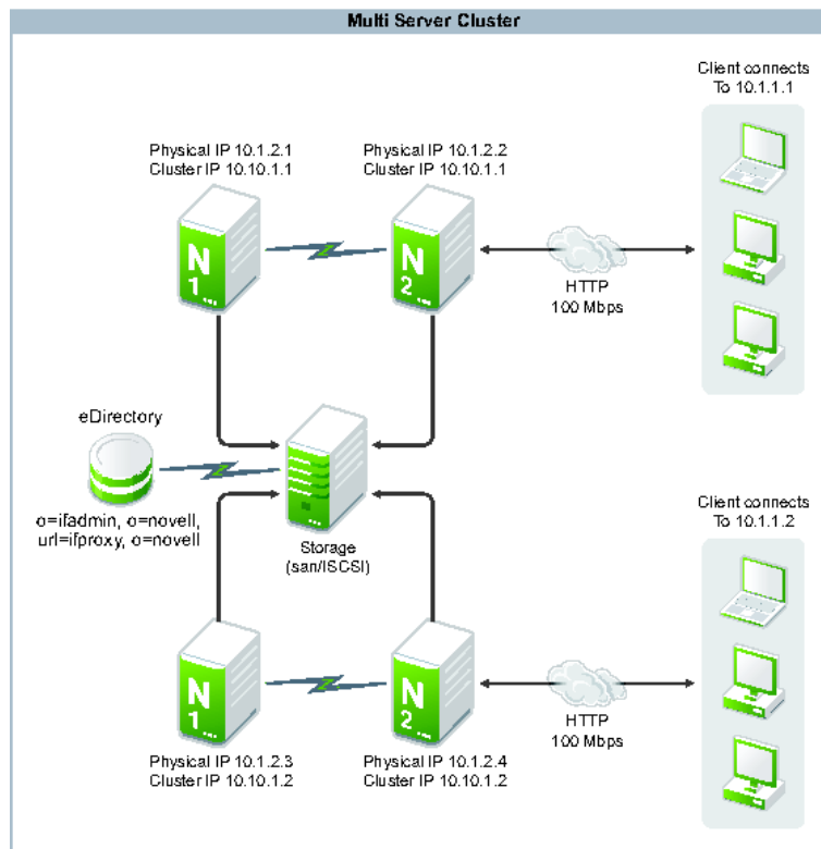
Figure 7-1 Multi-Server Cluster
