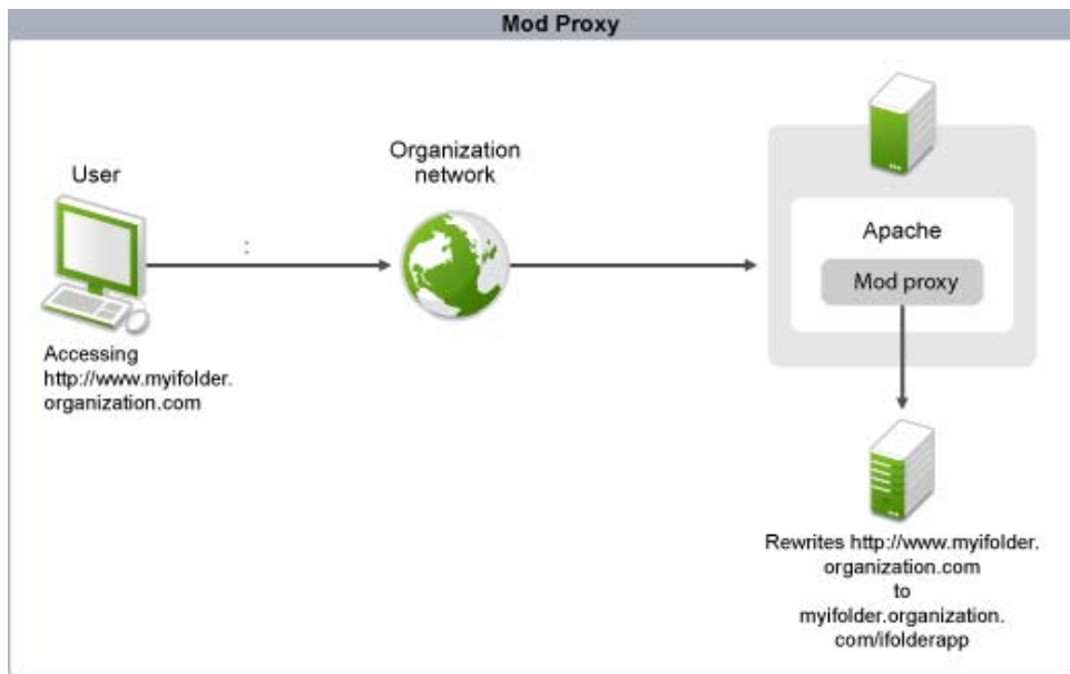
Figure 12-2 Mod Proxy
