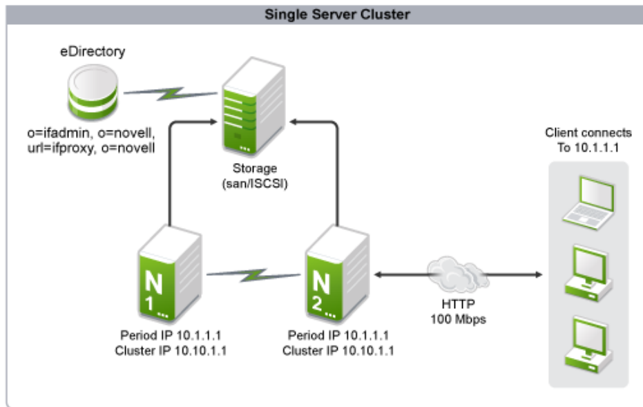
Figure 6-1 Single-Server Cluster
