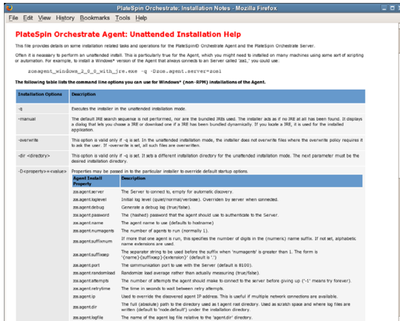
Figure 2-1 PlateSpin Orchestrate Agent Silent Installation Help
