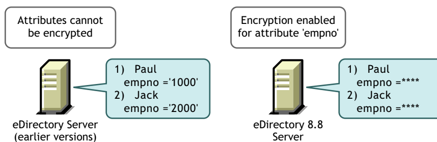
Figure 10-1 Encrypted Attributes
