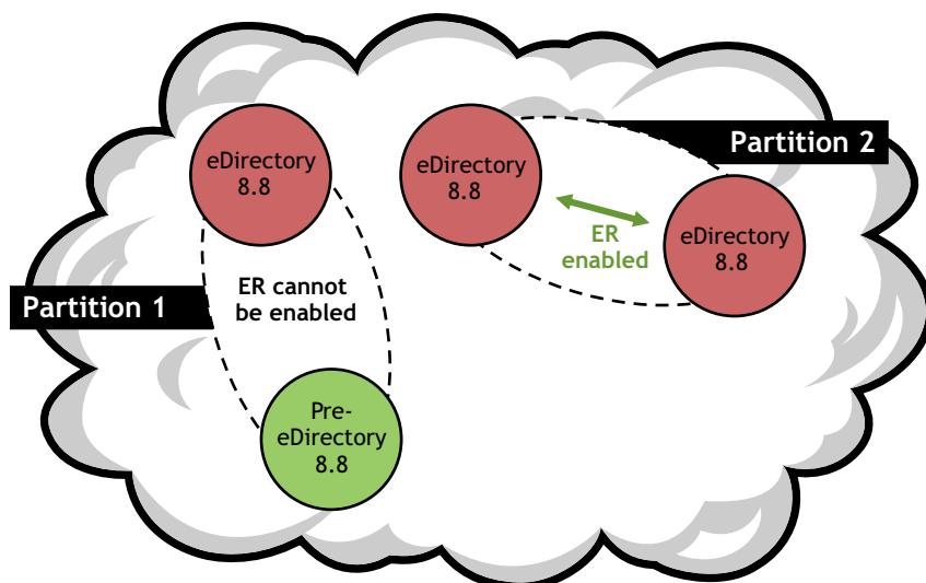
Figure 10-4 Encrypted Replication at Partition Level
