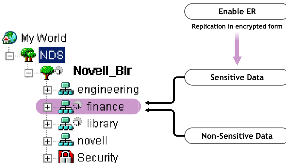
Figure 10-3 Encrypted Replication
