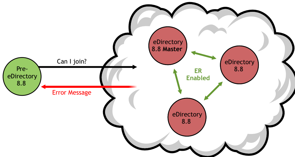
Figure 10-6 Adding Pre-eDirectory 8.8 Server to eDirectory 8.8 Replica Ring with Encrypted Replication Enabled.
