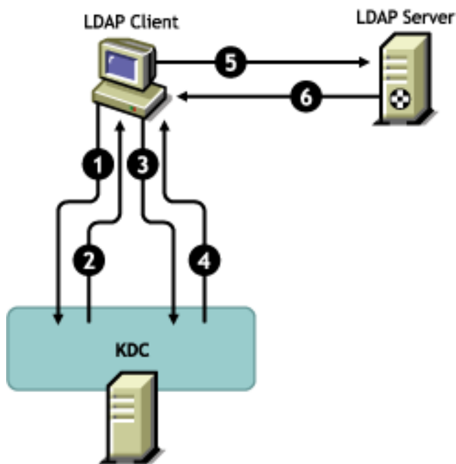
Figure 4-1 How GSSAPI Works?
