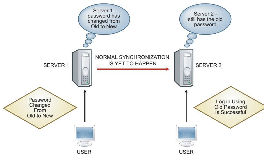
Figure 6-1 Need for Priority Sync
