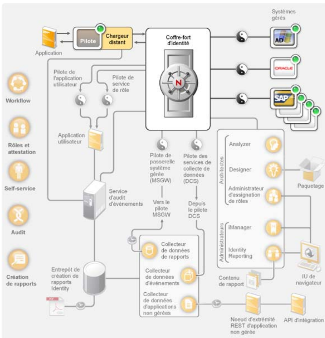
Figure 4-2 Composants de l'architecture Identity Manager
