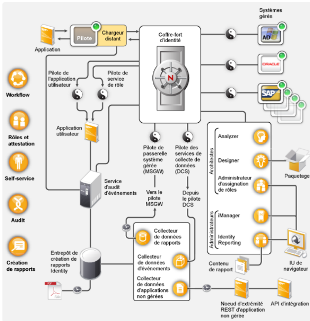
Figure 4-1 Architecture d'Identity Manager
