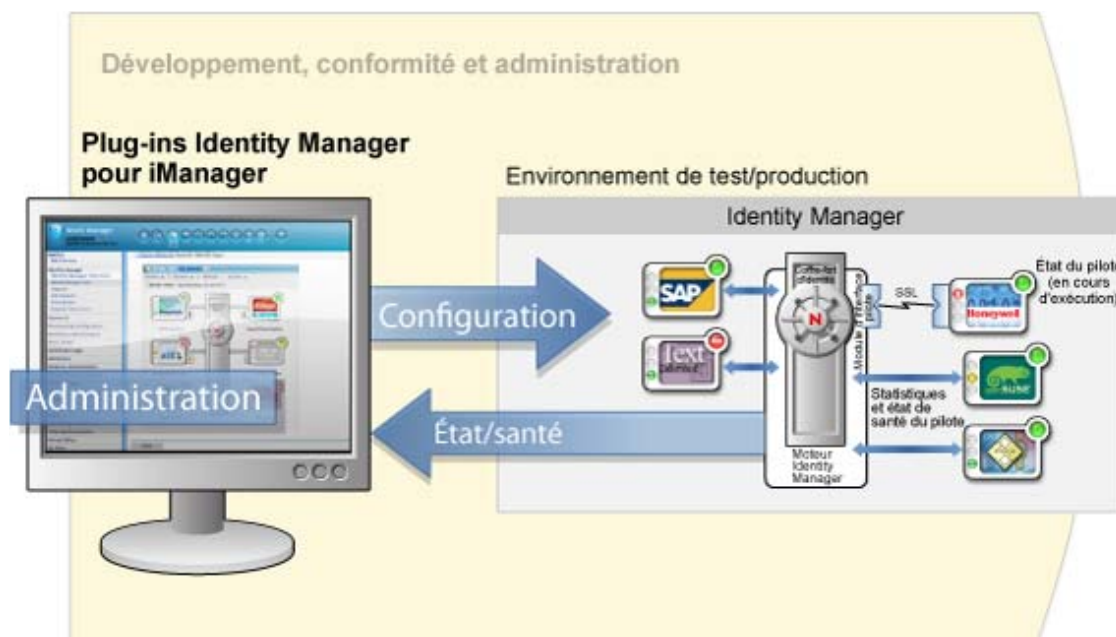
Figure 5-4 Novell iManager
