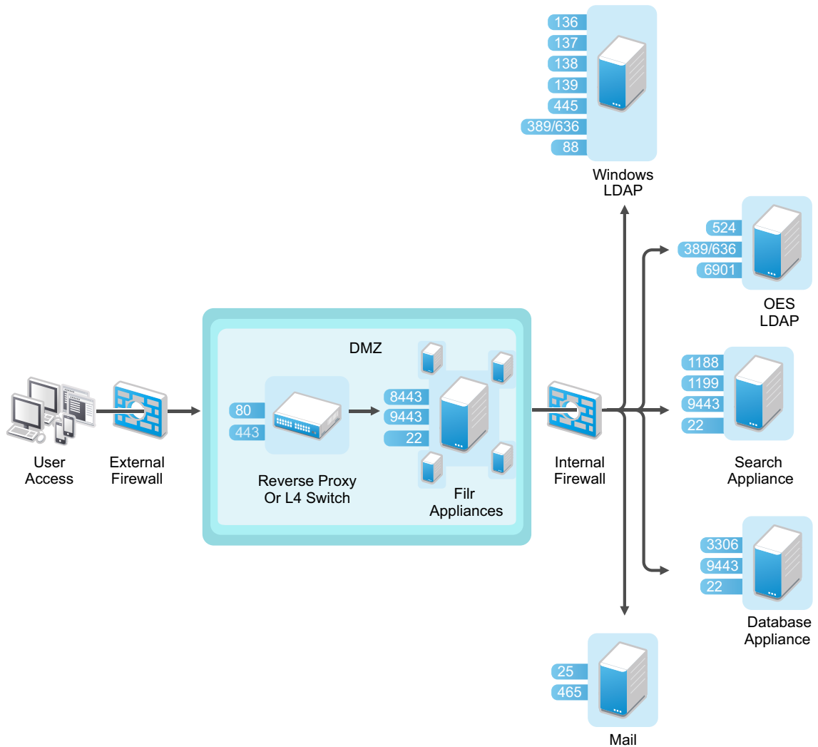
Figure 29-1 Filr in a DMZ
