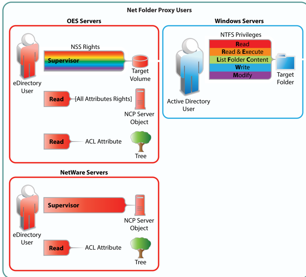
Figure 8-1 Net Folder Server Proxy User Rights Requirements
