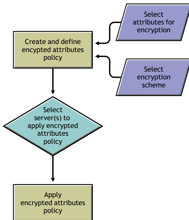
Figure 12-2 Encrypting Attributes
