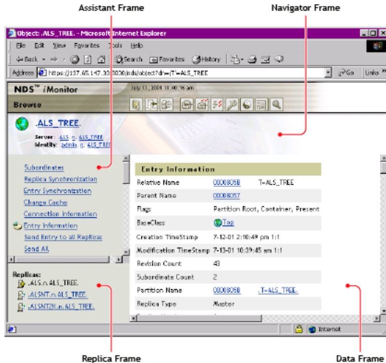
Figure 9-1 iMonitor Frames
