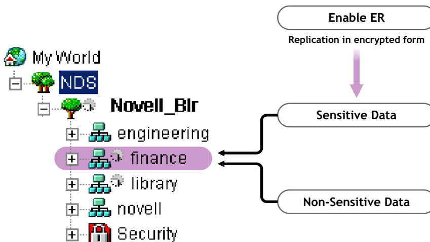
Figure 12-3 Encrypted Replication
