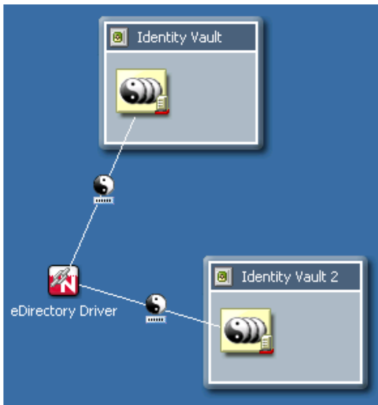
Figure 3-30 eDir-to-eDir Connections
