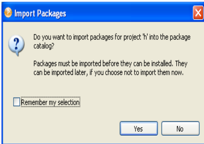
Figure 6-2 Importing Packages
