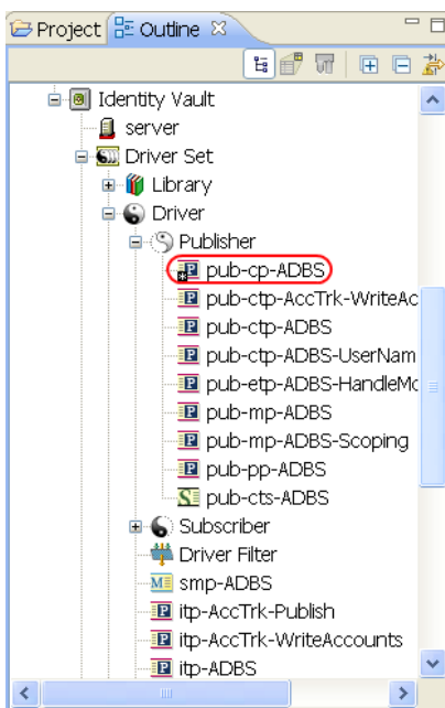
Figure 6-3 Changed Policy
