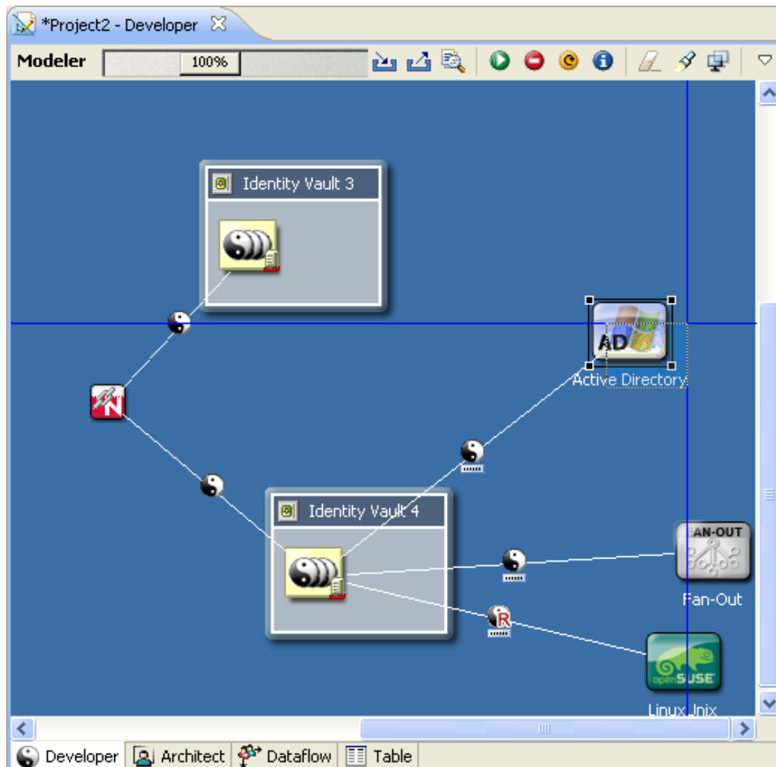
Figure 3-33 Alignment Hints
