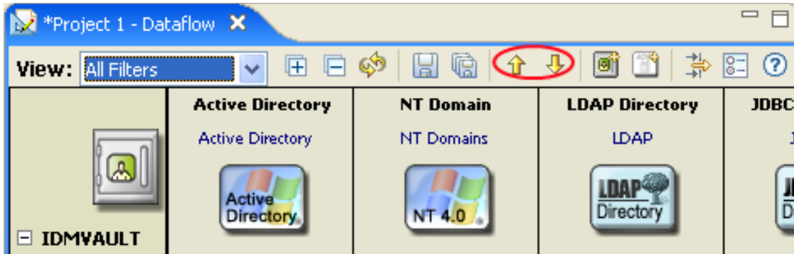
Figure 8-17 Navigation Icons
