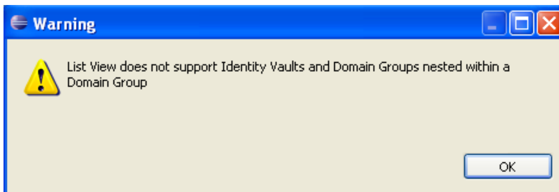
Figure 3-25 Warning Message
