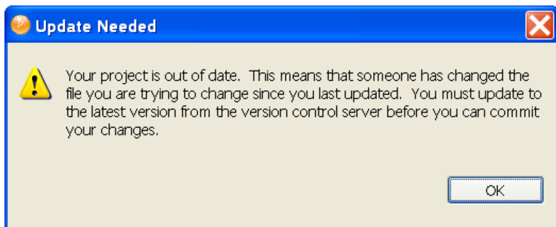
Figure 20-17 Conflict Message
