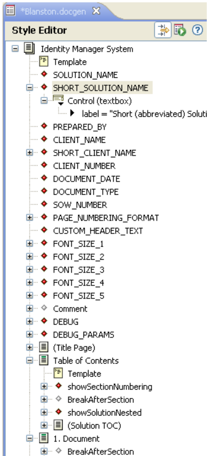
Figure 13-7 Attributes
