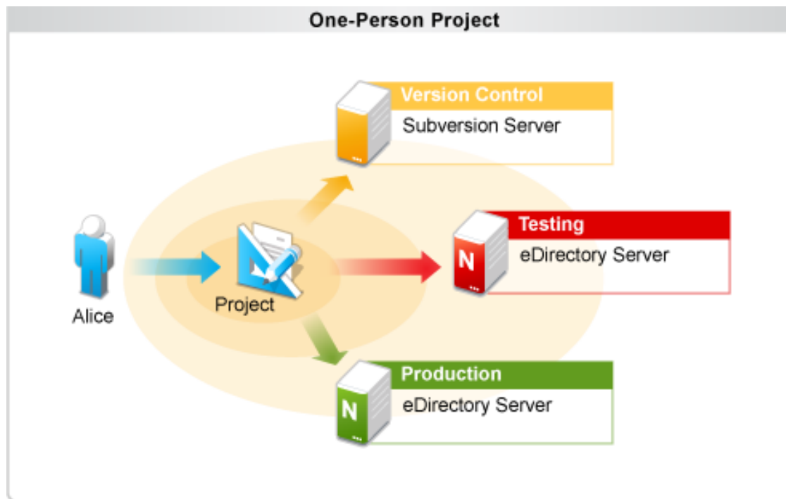
Figure 20-26 One-Person Project
