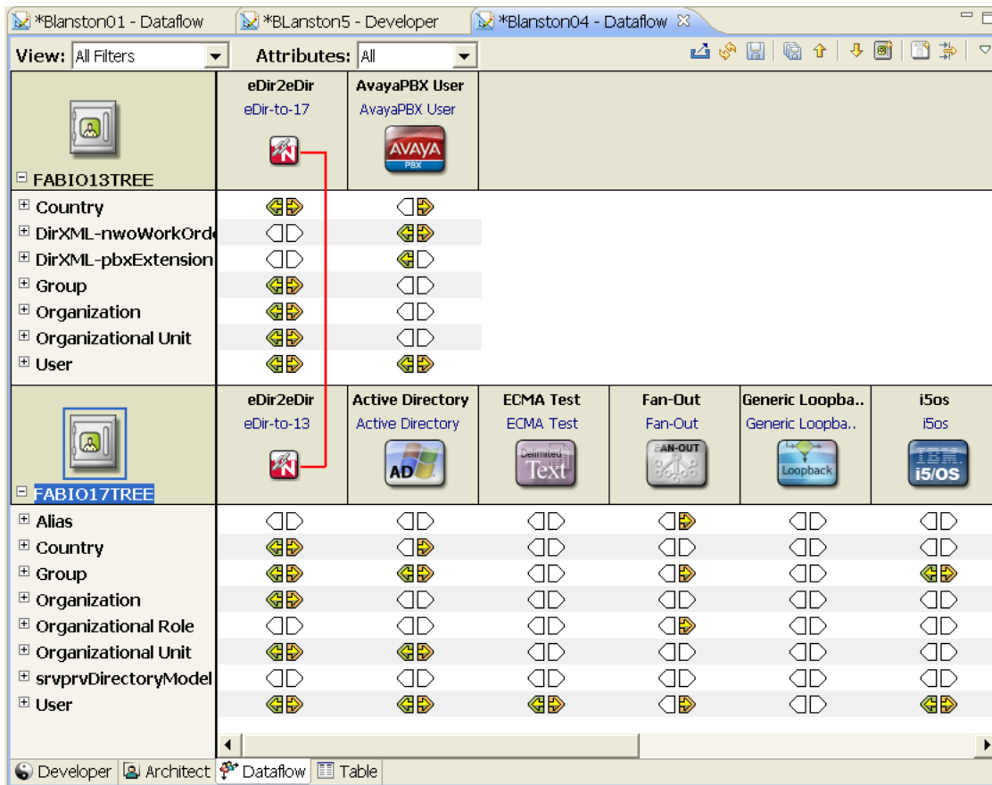
Figure 3-8 Dataflow Mode
