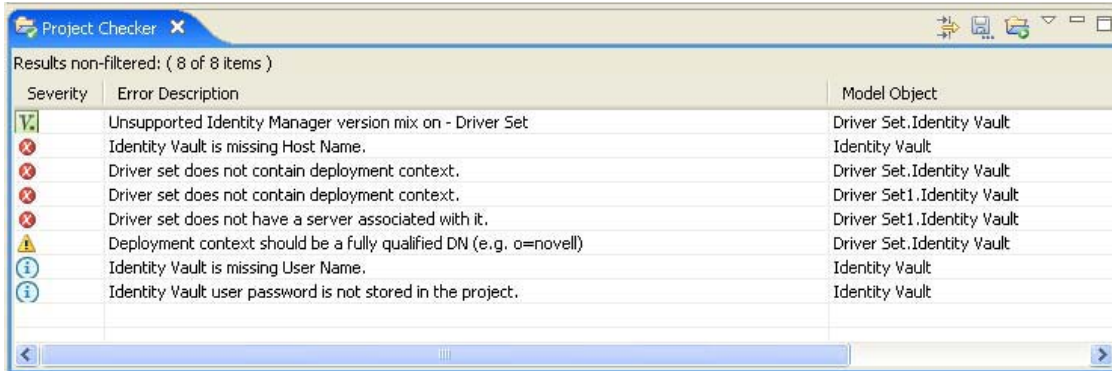
Figure 5-6 Project Checker
