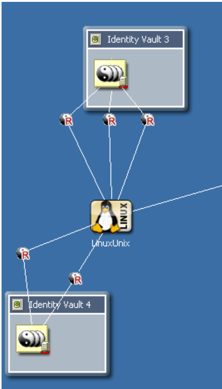
Figure 3-31 Multi-Driver Connections
