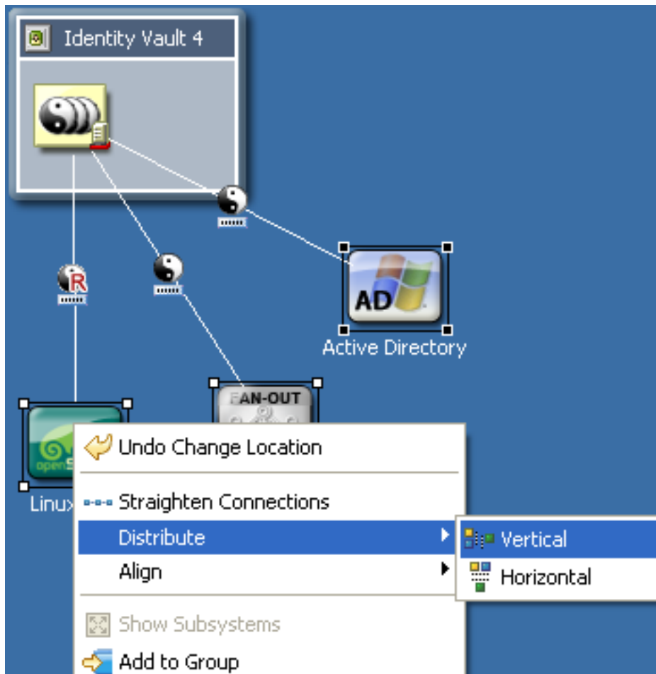
Figure 3-35 Distributing Applications
