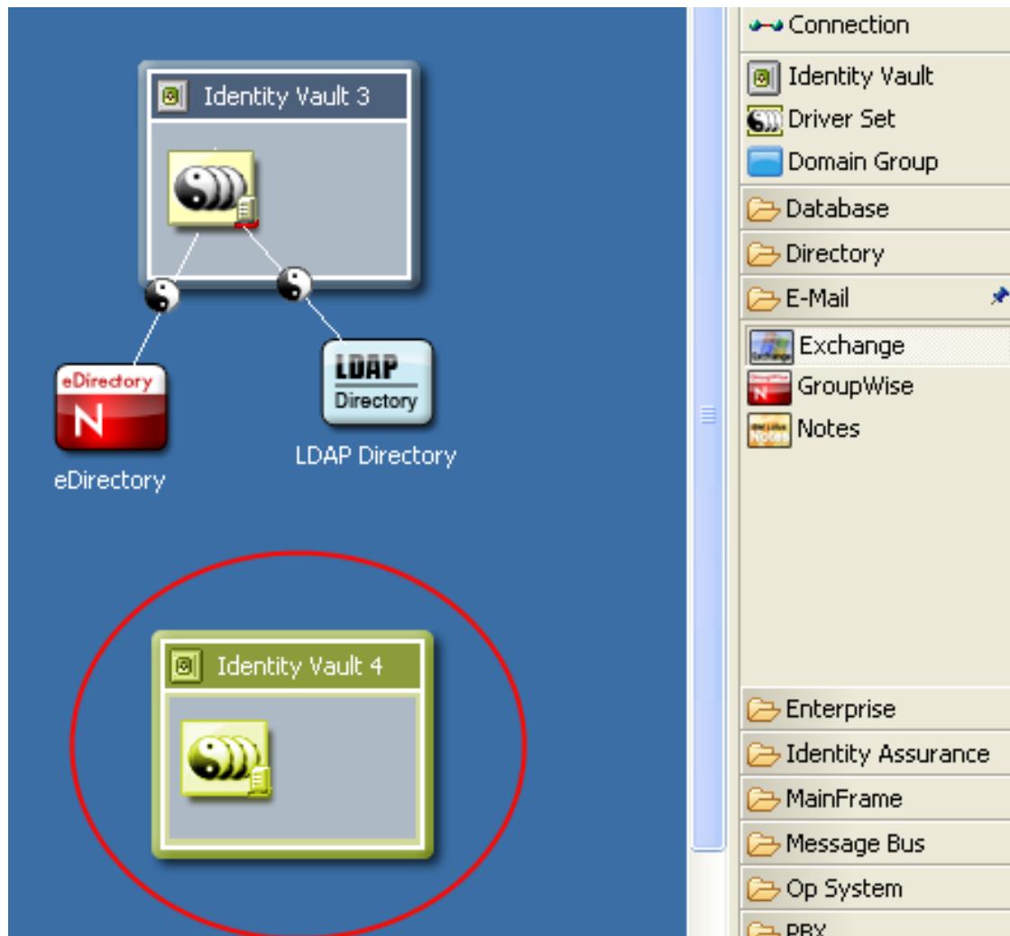
Figure 3-29 Connected Objects
