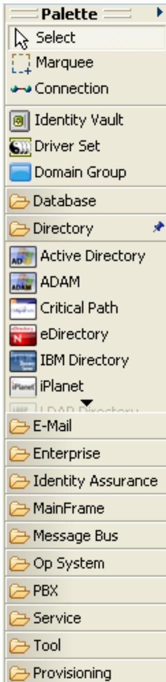
Figure C-1 Designer's Palette
