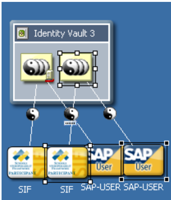
Figure 3-15 Driver Sets
