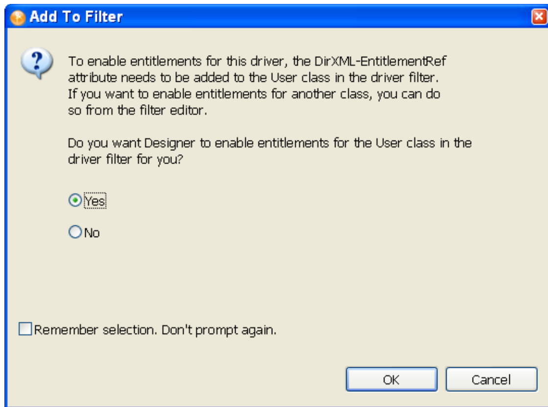
Figure 14-2 Enabling Entitlements
