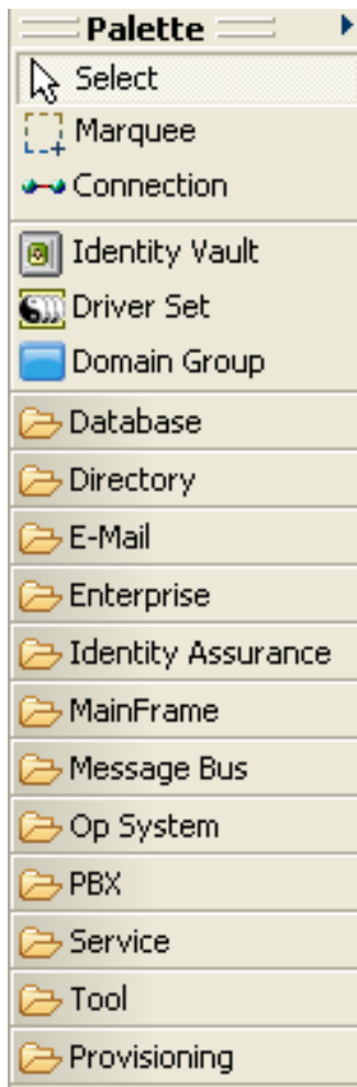
Figure 3-10 Designer’s Palette
