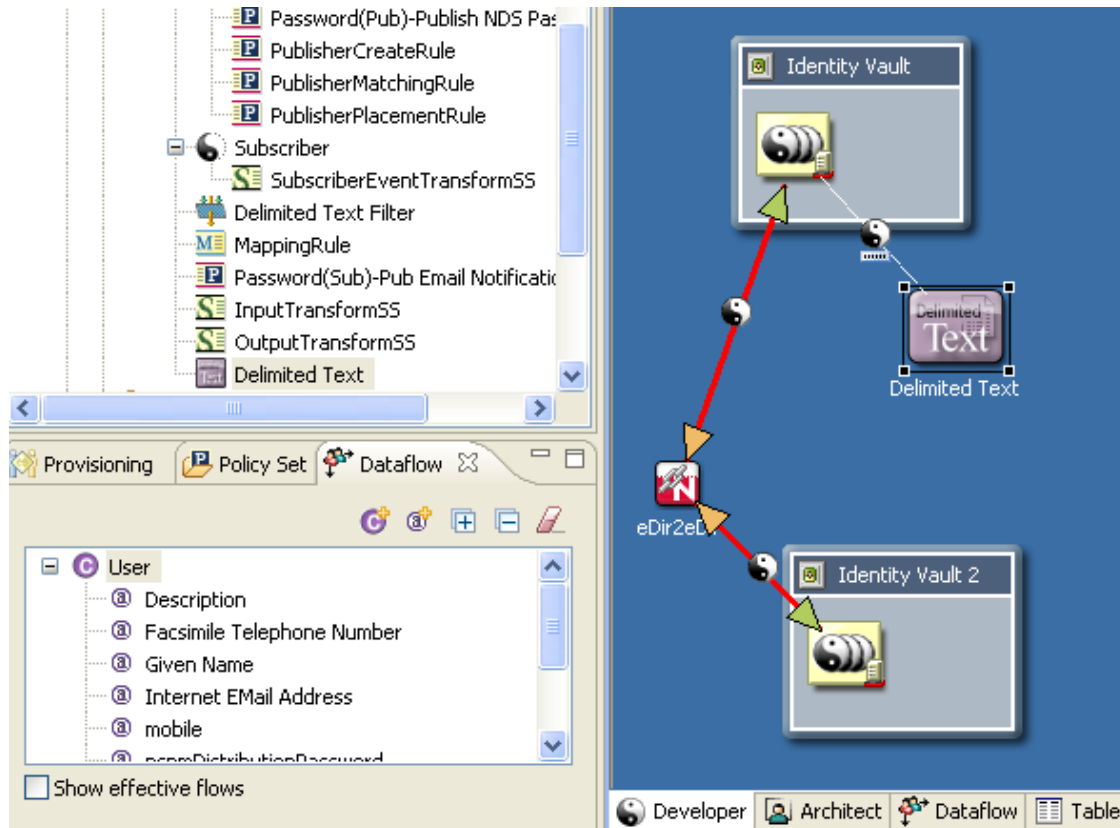
Figure 8-3 Flow Arrows in the Modeler
