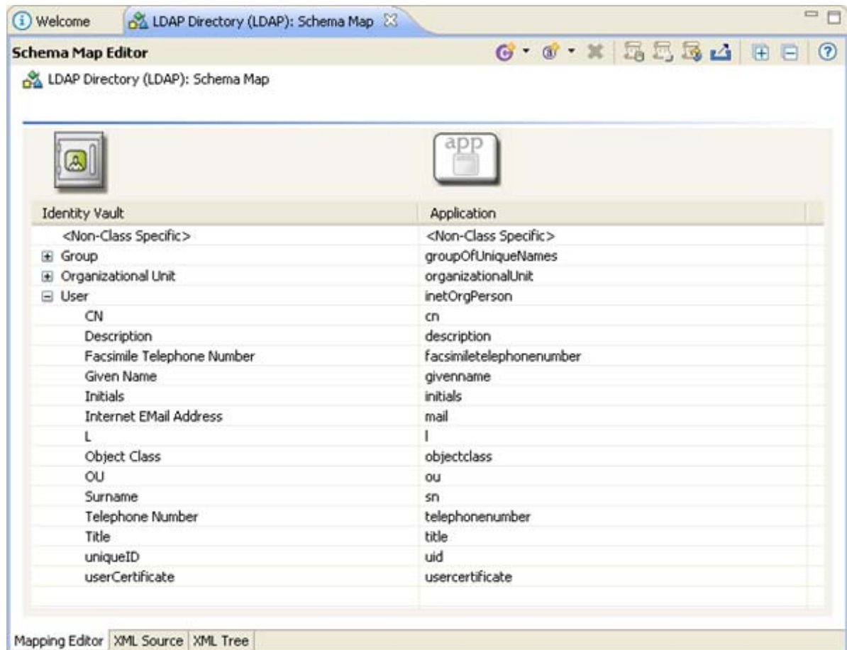
Figure 1-4 Schema Map Editor
