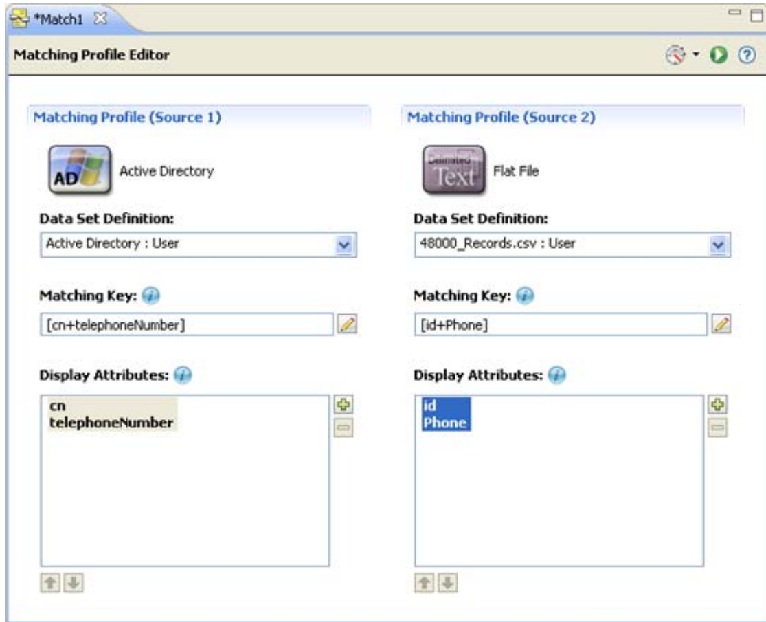
Figure 1-11 Matching Profile Editor
