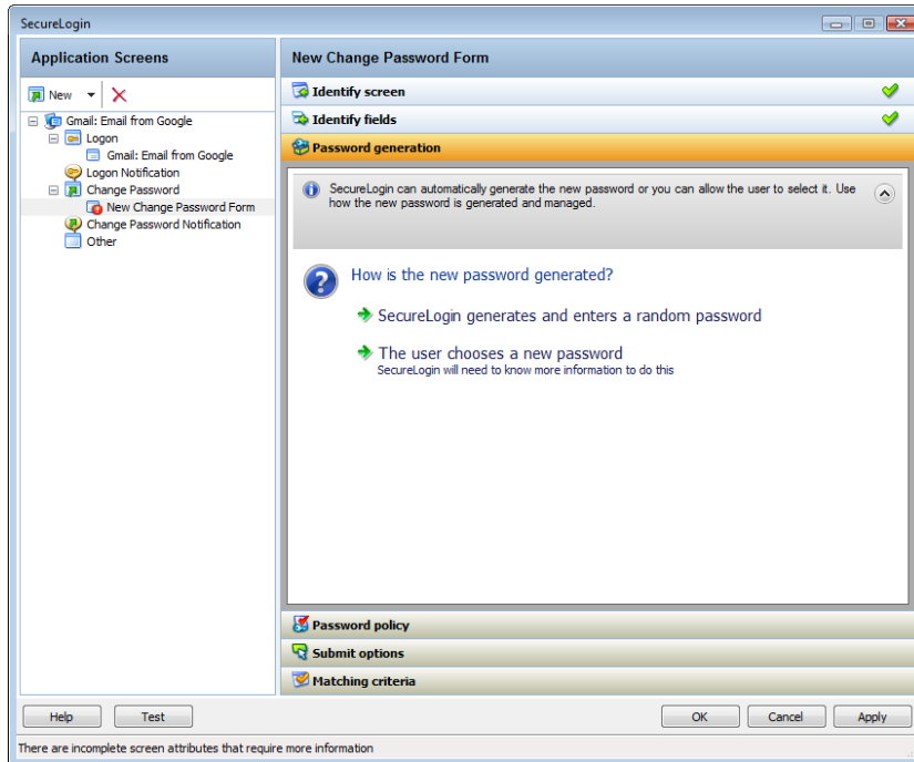
Figure 2-11 The Password Generation Options
