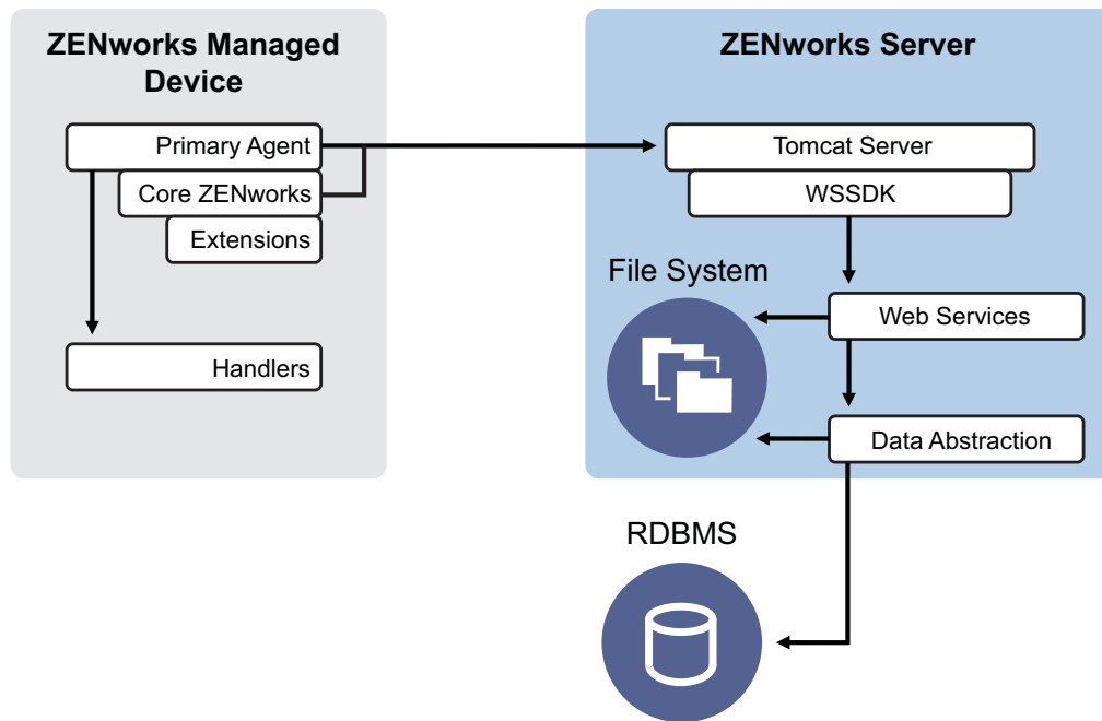
Figure 2-3 ZENworks 11 Client-Server Architecture
