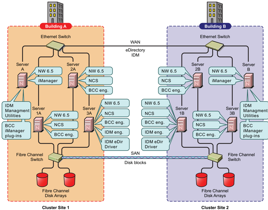
Figure 2-1 Business Continuity Cluster Component Locations
