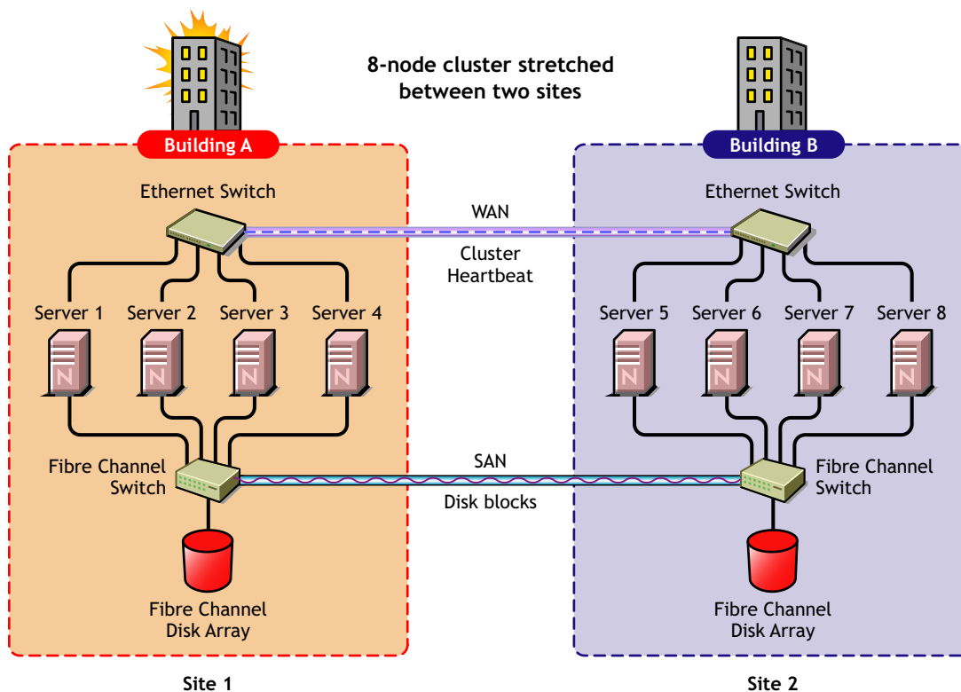
Figure 1-1 Stretch Cluster
