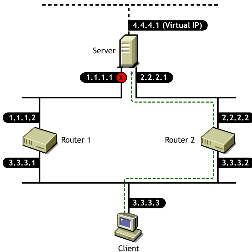
Figure 5-2 Multihomed Server Using Virtual IP Addresses
