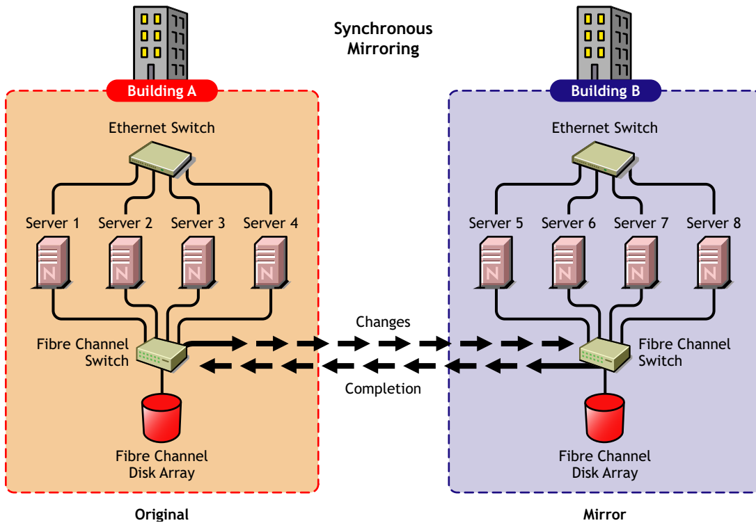
Figure 2-2 Synchronous Mirroring
