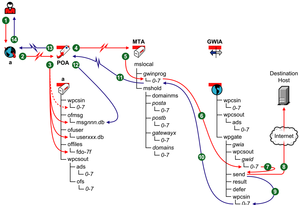
Figure 4-3 Message Flow When the Mapped Link is Open
