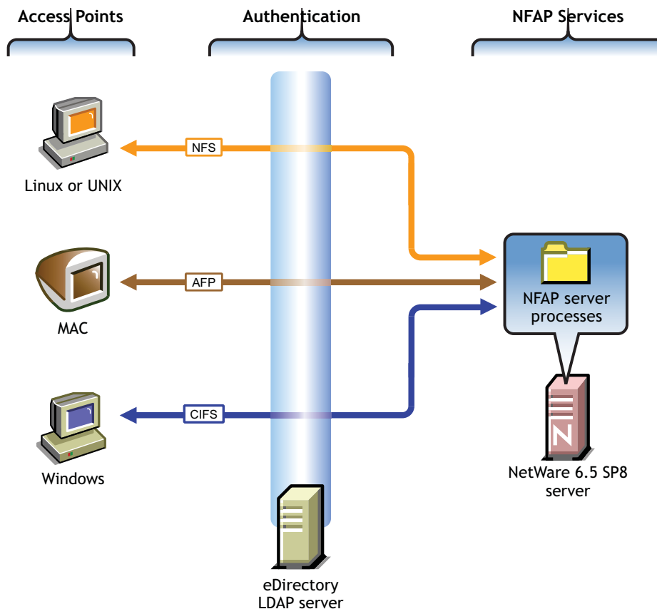
Figure 7-1 Native File Access Support on NetWare 6.5
