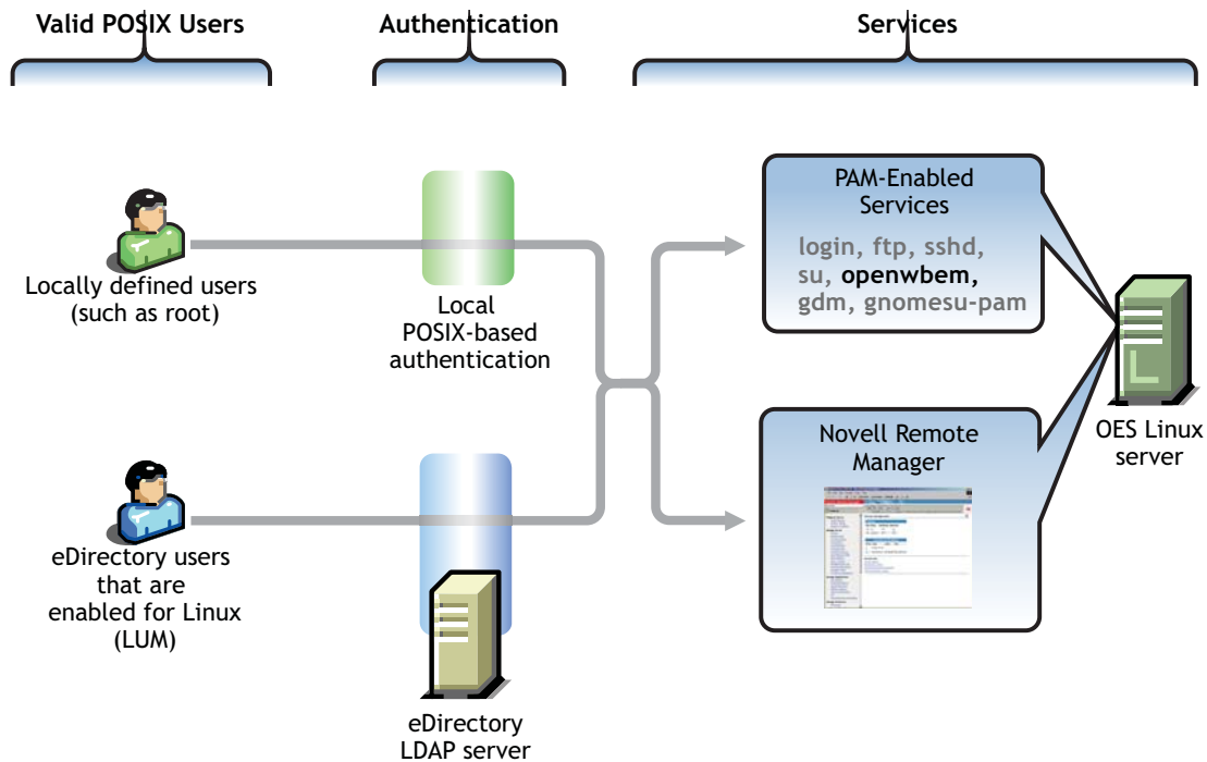
Figure 4-1 Linux User Management on OES
