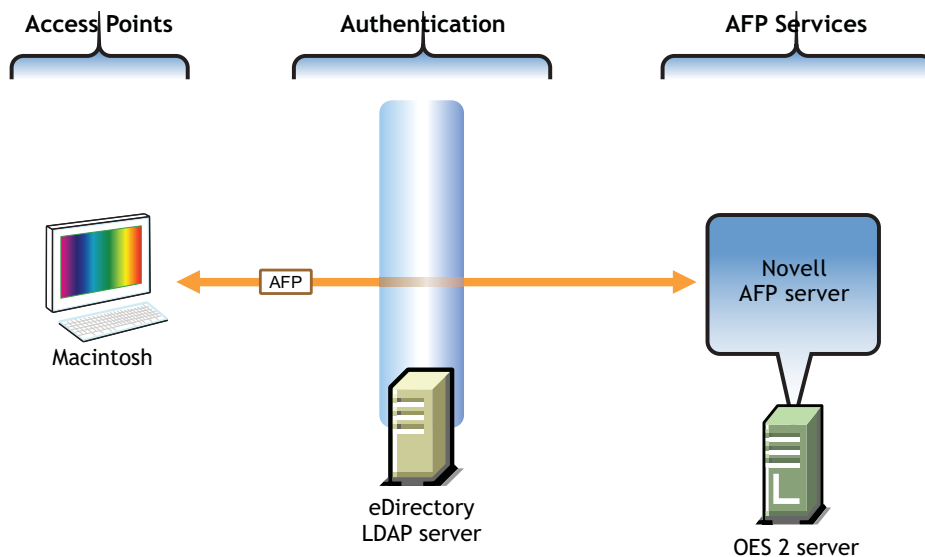
Figure 6-1 AFP File Access Support on OES 2
