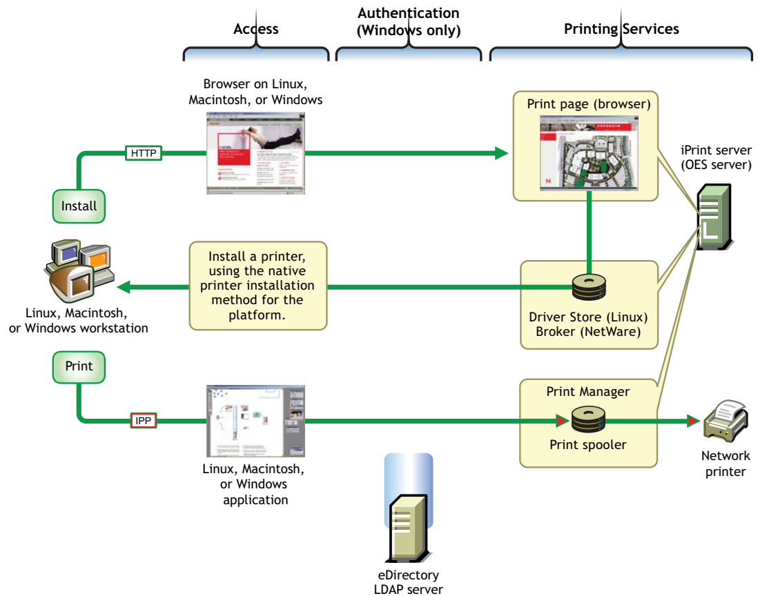
Figure 9-1 iPrint on OES
