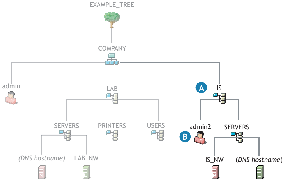
Figure 3-3 An Expanded Tree
