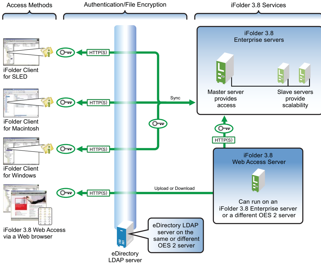
Figure 8-1 iFolder File Services on OES
