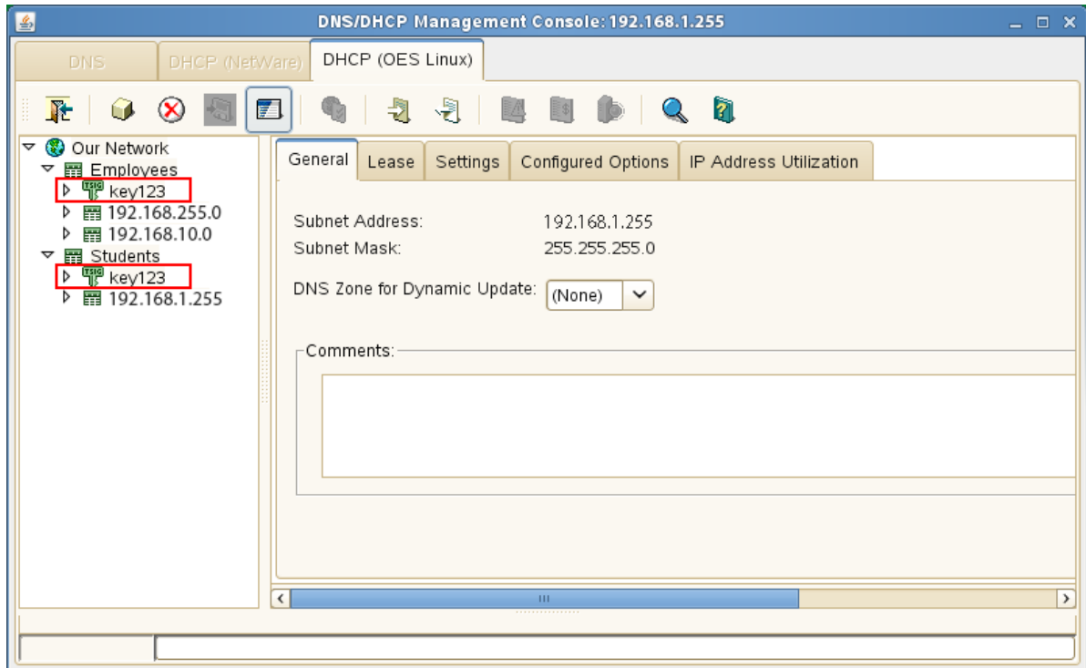
Figure 18-1 Management Console
