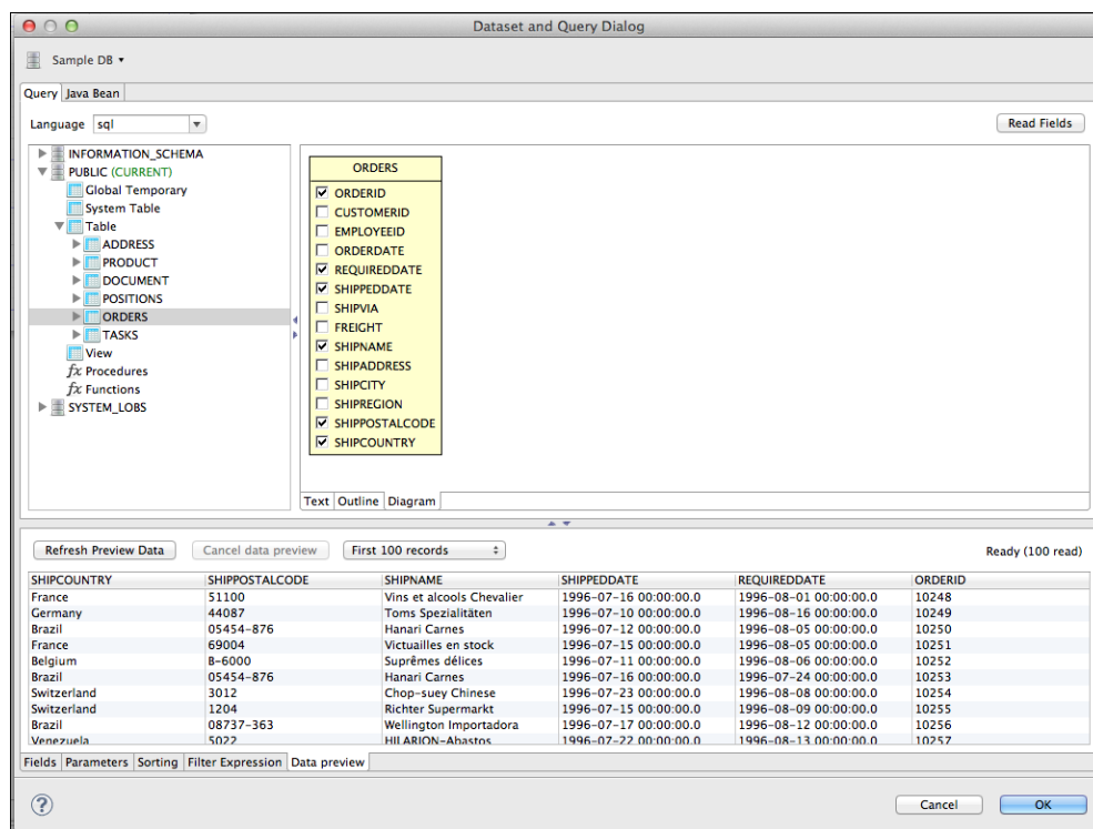
Figure 18-10 Data Preview Tab
