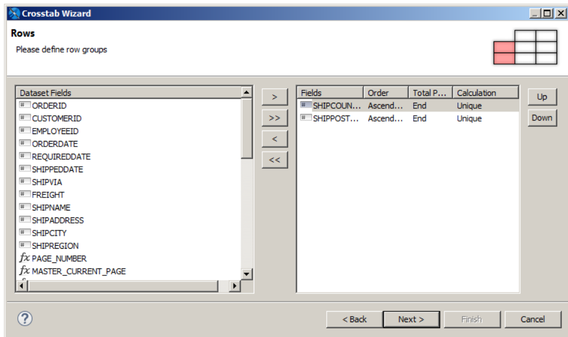
Figure 13-5 Defining row groups
