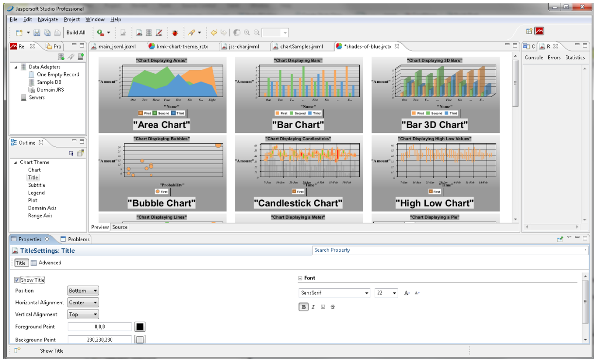
Figure 5-16 A Chart Theme Edited in Jaspersoft Studio
