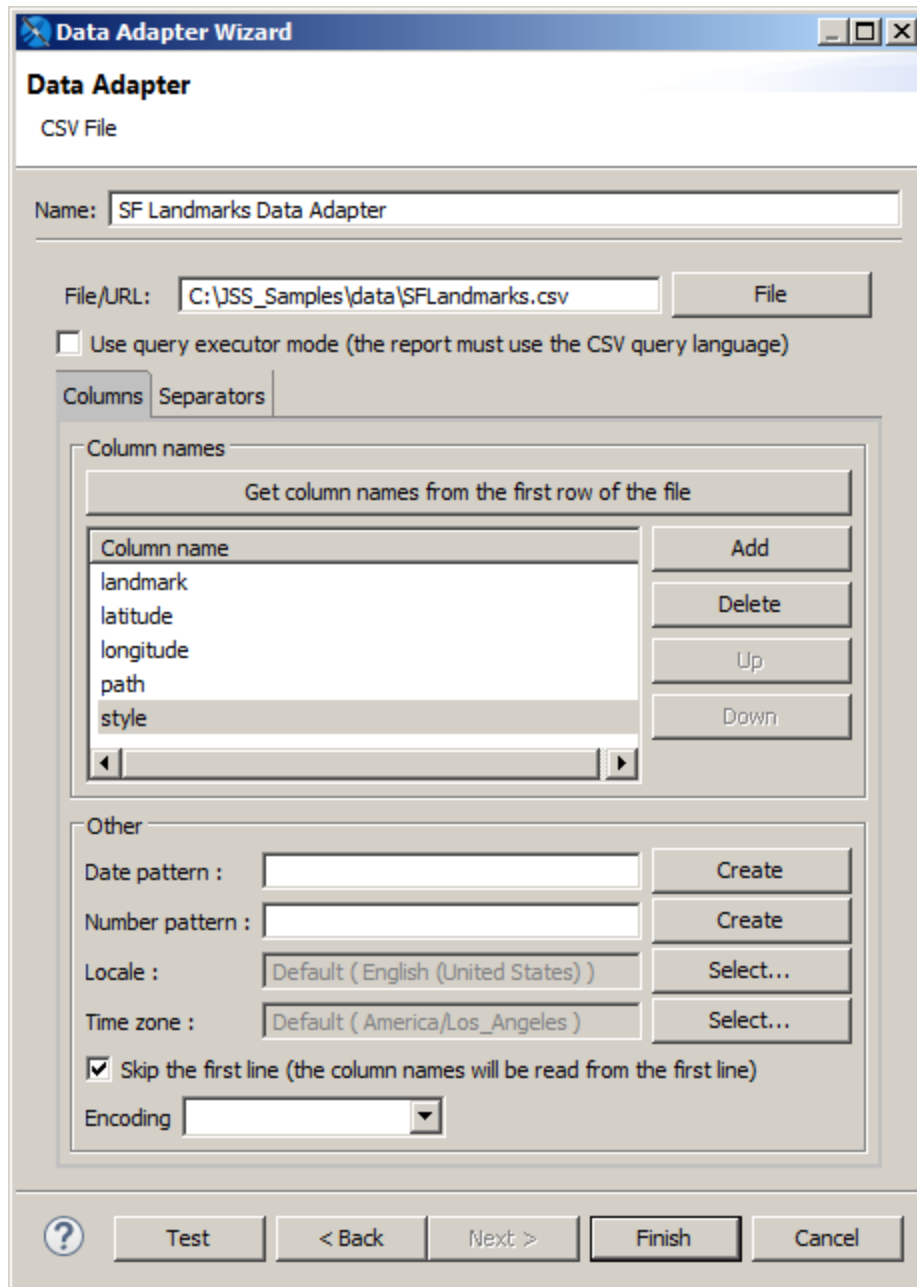
Figure 10-22 CSV Data Adapter
