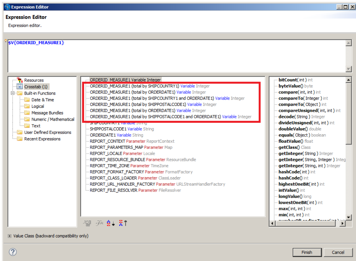
Figure 13-18 Total variables in the expression editor
