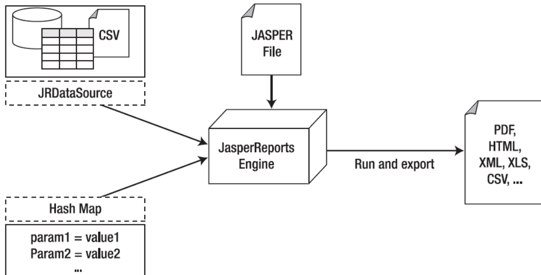
Figure 2-1 Data Source and Parameter Flows for Report Creation
