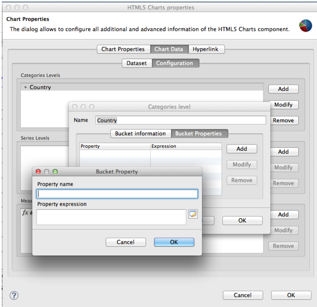
Figure 14-21 Defining Bucket Properties for HTML5 Chart Hyperlinking
