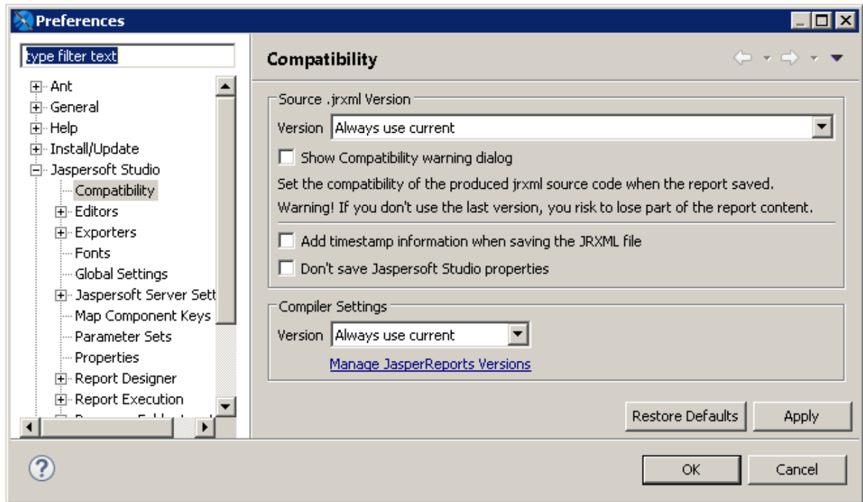
Figure 2-2 Setting JasperReports Library Version
