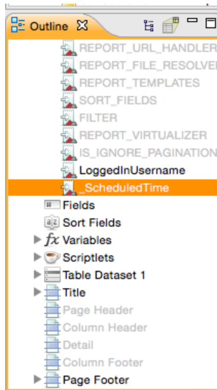
Figure 5-18 _ScheduledTime Parameter in Outline View
