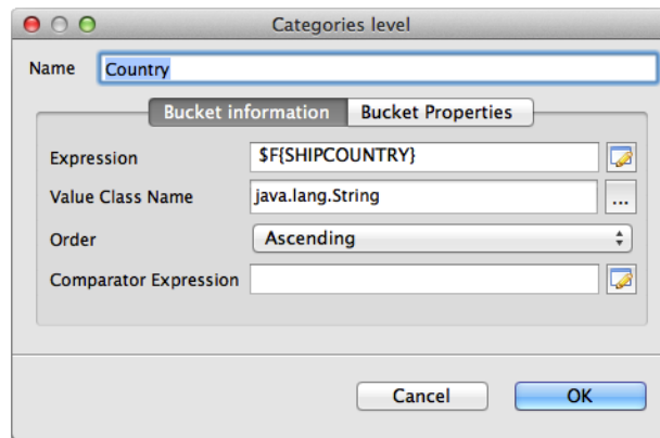
Figure 14-15 Editing Categories in the Chart Data Configuration Window
