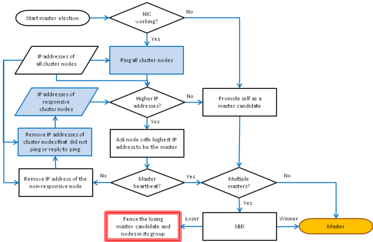
Figure C-2 Master-Election Algorithm for OES 11 SP1 and Later (and Fully Patched OES 11 and OES 2 SP3)
