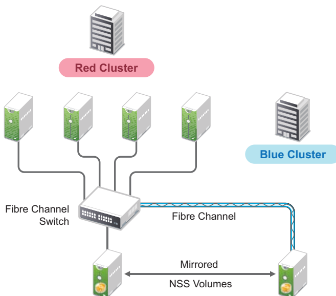
Figure 13-2 Single Cluster with Mirrored NSS Volumes in Separate Buildings
